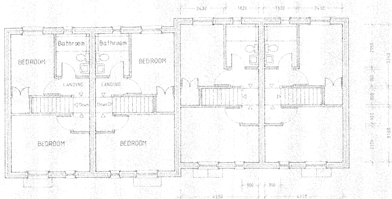
PROPOSED FIRST FLOOR PLANS.
