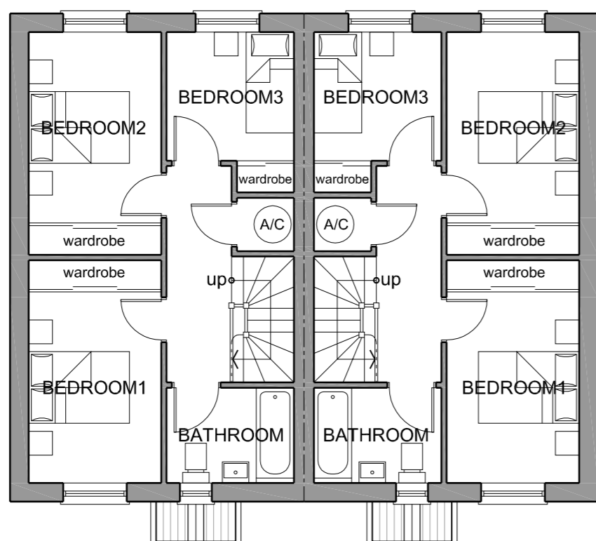
FIRST FLOOR PLAN (GIA 85sqm/914sqft)
